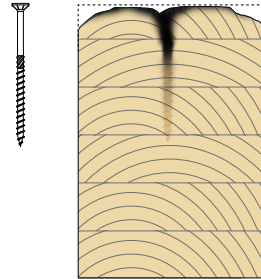
Ø12 (0.48 in) screw with head exposed to a heat source
