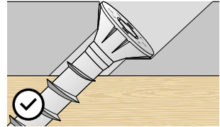
Inclined countersunk hole
