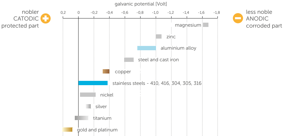
Galvanic series of metals: corrosion potential of various metals in salt water
