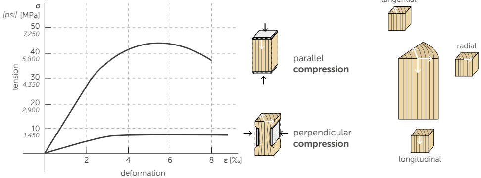
Typical stress-strain curves
