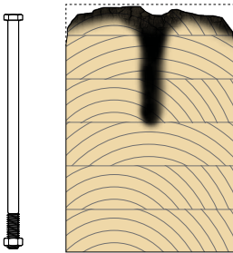
Ø20 (0.79 in) bolt exposed to a heat source
