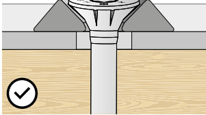
Flared washer.
