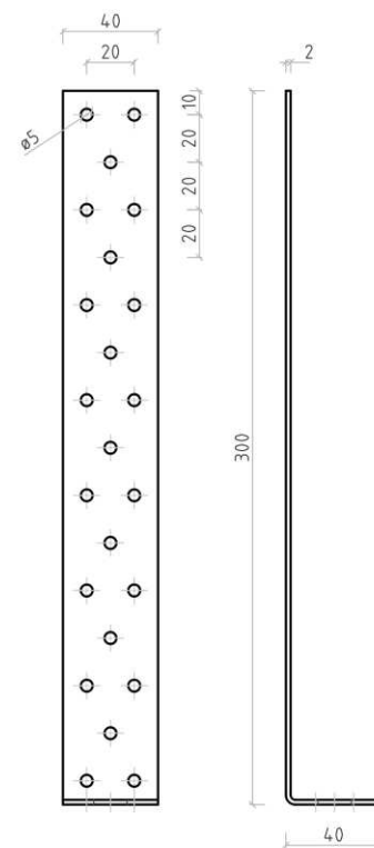
Figure B. 2 Dimensions of type WZU2002
