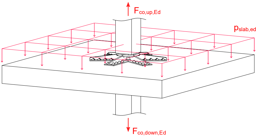
Figure A3.1: Forces and loads on the SPIDER Connector
