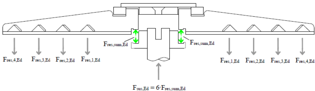
Figure A3.2: Load case 1 – Forces from p_{\text{slab,ed}} on the CLT
