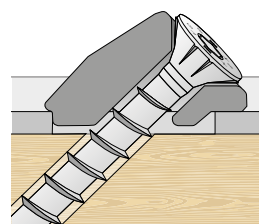
Slotted hole with VGU washer.
