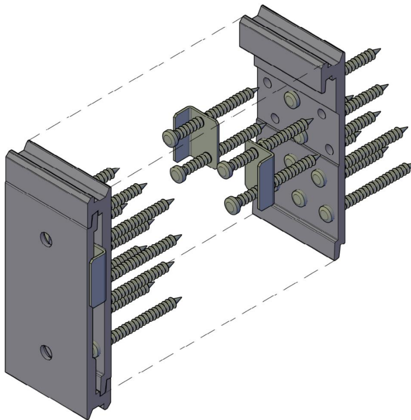
Figure 3 LOCK C connector with lateral locking system
